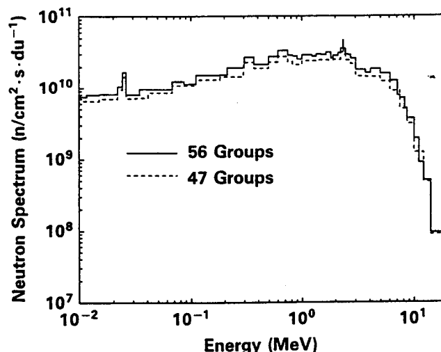
Fig. 6. The ELXSIR and BUGLE-80 neutron spectra at the pressure vessel inner wall surface for SONGS-2.
