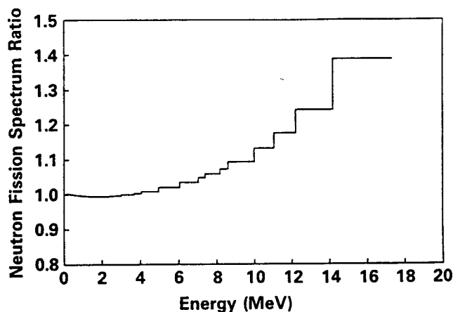
Fig. 8. The ratio of a mixed fission spectrum (16.5% ^{239}\text{Pu} and 83.5% ^{235}\text{U} ) to that of a pure ^{235}\text{U} fission spectrum.
