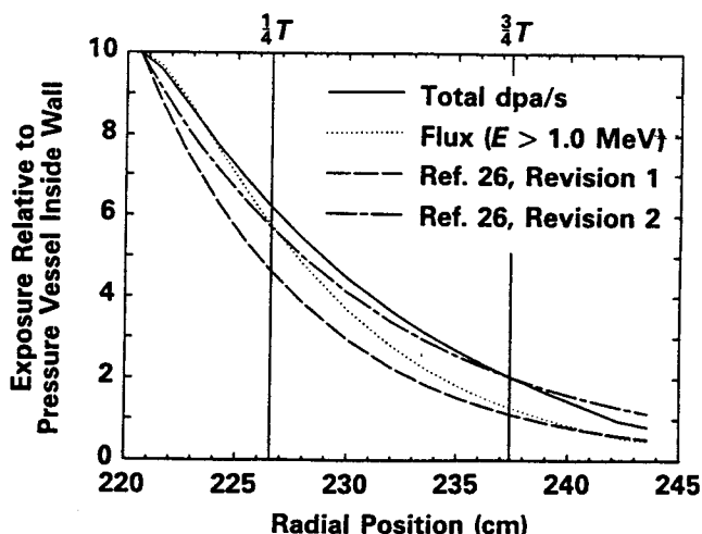
Fig. 12. A comparison of the attenuation of several key exposure parameters through the pressure vessel wall of SONGS-2.
