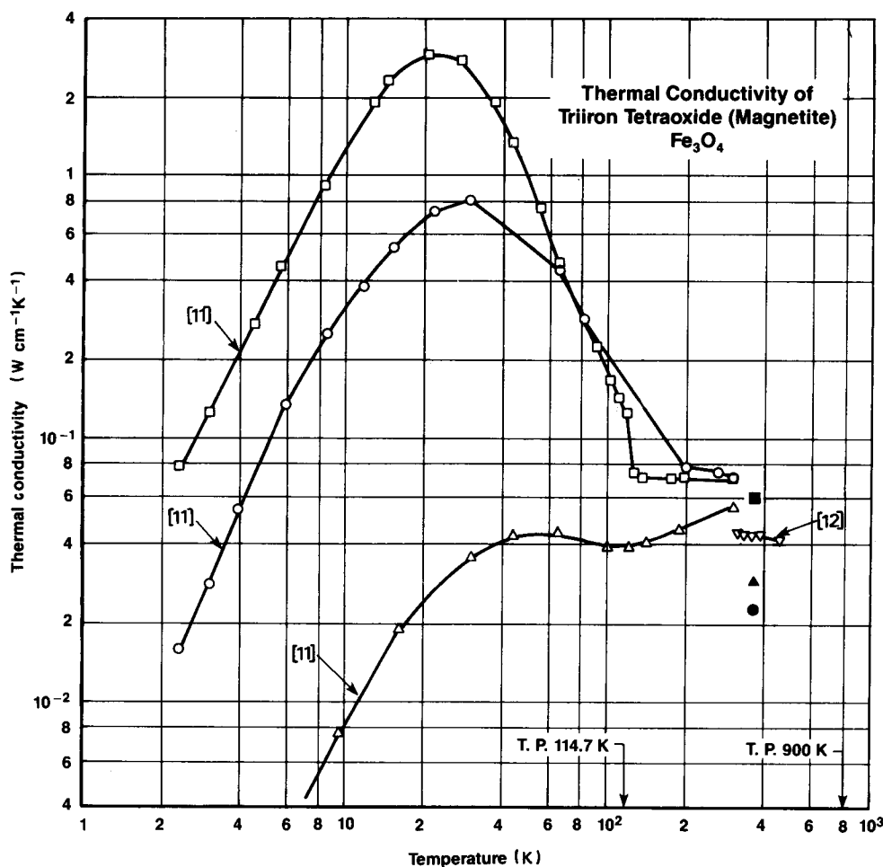
Figure 3 Comparison of Oconee miniature flake thermal conductivity data with Fe 3 O 4 data (from ref. 10). Specimens ▲, B; ●, G; ■, H.
