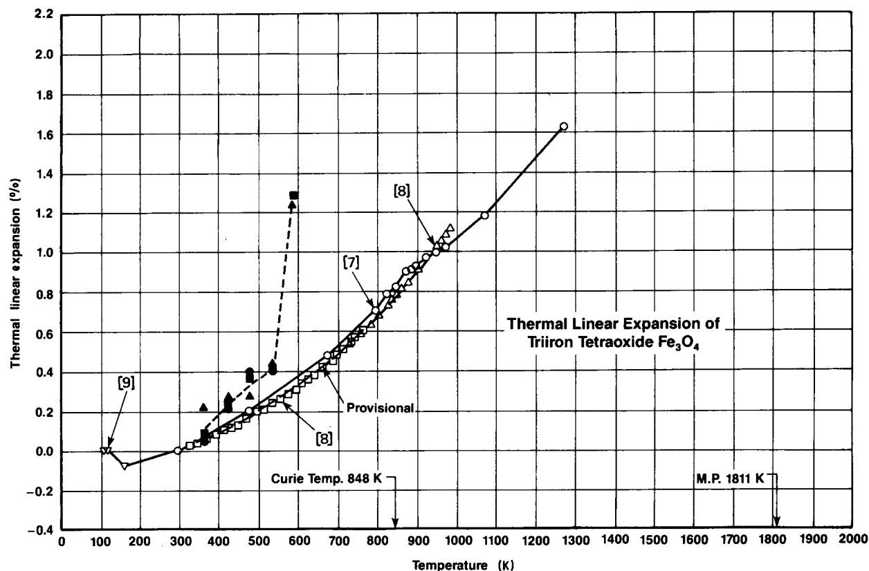
Figure 1 Comparison of Ocone miniature flake thermal expansion data with \text{Fe}_3\text{O}_4 data (from ref. 6). Specimens \Delta , A; \bullet , G; \blacksquare , H; ---, fit to miniature flake data.
